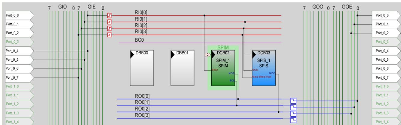
Figure 10. Example PSoC Designer Routing of a “Loopback” System
