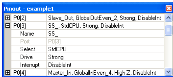
Figure 9. Example SS_ GPIO Configuration
