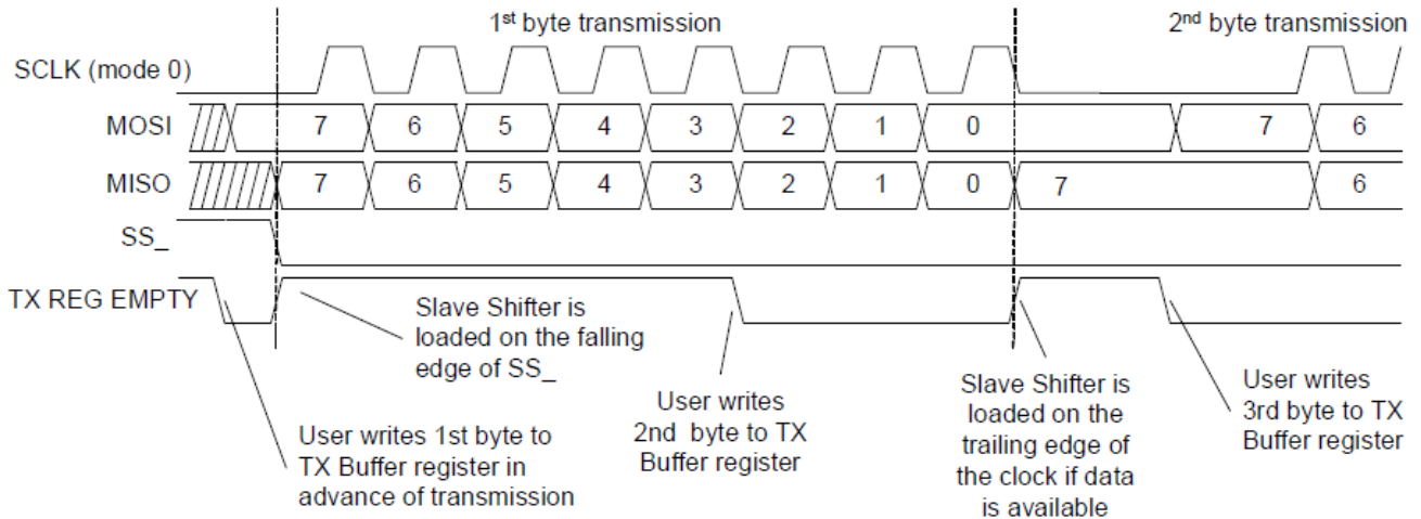
Figure 18. Shifter Loads in Mode 0 and 1 without SS
