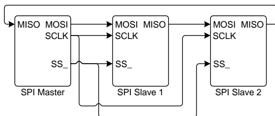
Figure 11. Daisy-Chained Multiple Slave System
