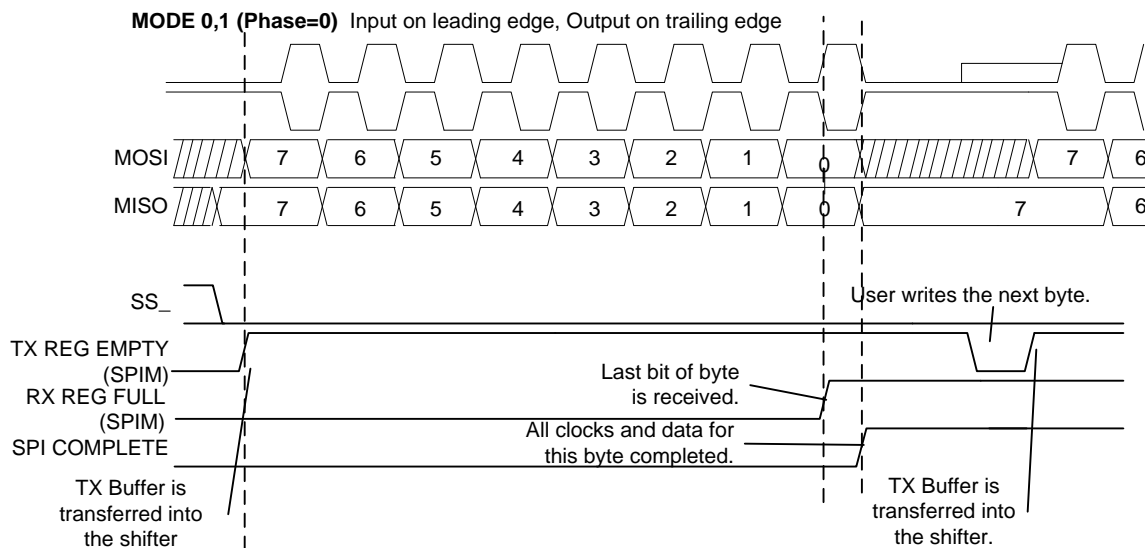
Figure 6. Mode 0, 1 Status
