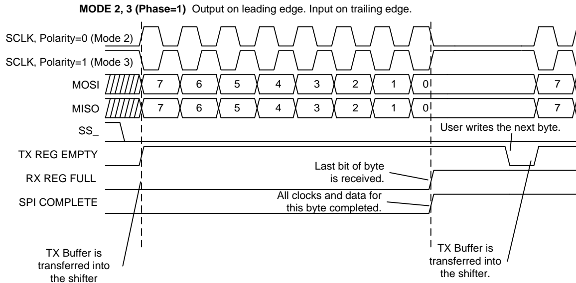
Figure 7. Mode 2, 3 Status
