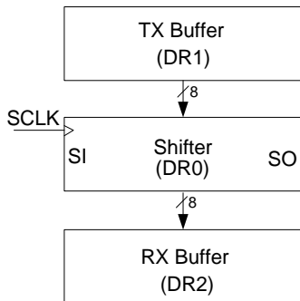
Figure 5. SPI Functionality in Digital Blocks
