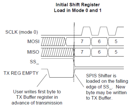
Figure 16. Initial Shifter Load for Mode 0 and 1
