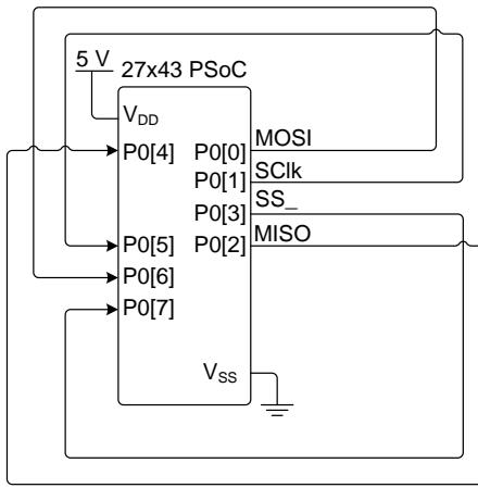
Figure 20. Physical Configuration for Example 1
