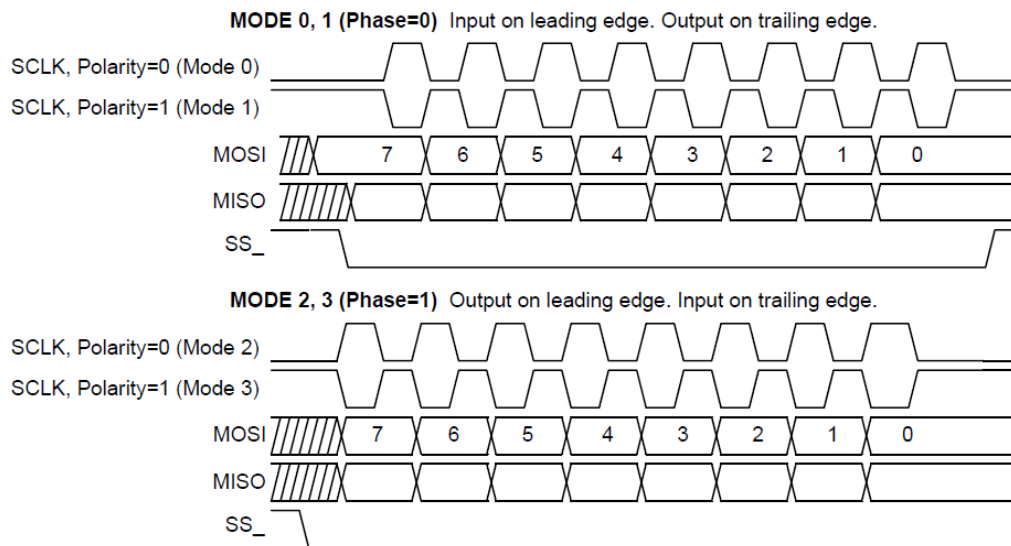
Figure 3. SPI Timing by Mode
