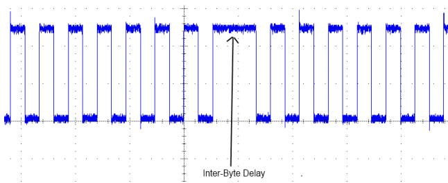
Figure 15. Interbyte Delay
