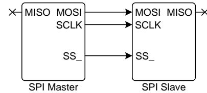
Figure 2. Two-Device Simplex SPI System Block Diagram
