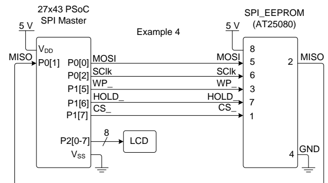
Figure 22. Physical Configuration for Example 4
