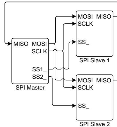
Figure 12. Parallel Multiple-Slave System
